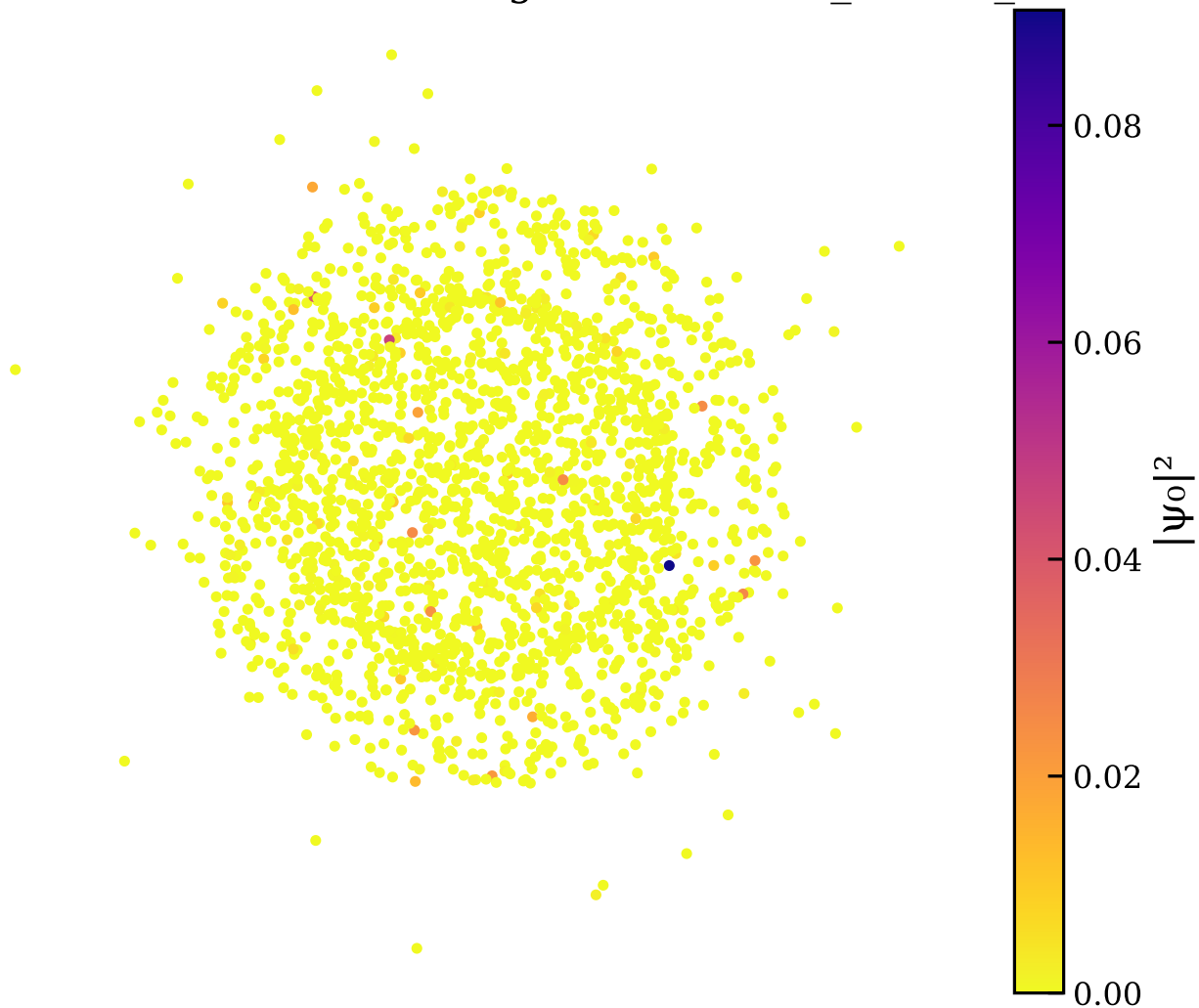
Ground state distribution: configuration model_N2000_G2
